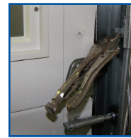
Lift into opening, level, fit top corner fasteners and lock top section.
